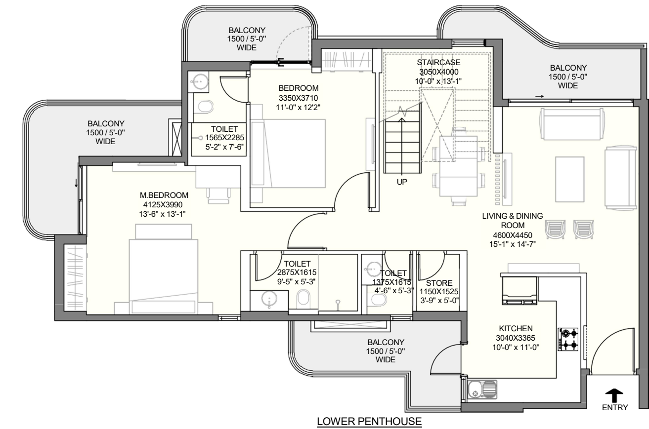
LOWER PENTHOUSE
