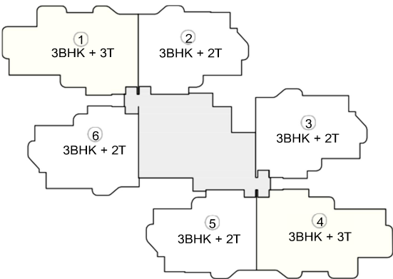
HARMONY TYPICAL FLOOR (1ST-17TH , 19TH-26TH & 28TH- 30TH FLOOR)
