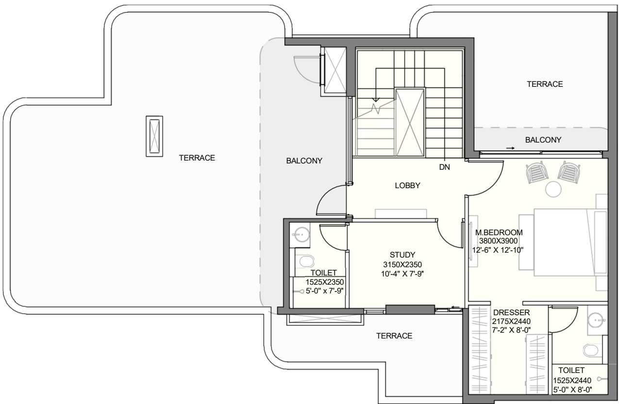
UPPER PENTHOUSE
